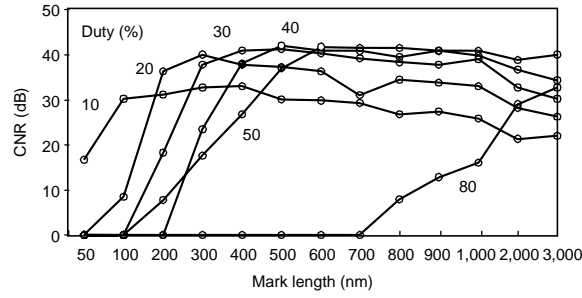
Fig. 5.60. Relationship between CNR and mark length for super-RENS readout ( P_r = 4 \text{ mW} ), with optical pulse duty as parameter
