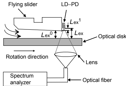
Fig. 2.8. Proposed set up for measurement of wavelength tuning based on ESEC length. An LD attached to an air-bearing slider flies by air resistance caused by disk rotation (upside down in reality)
