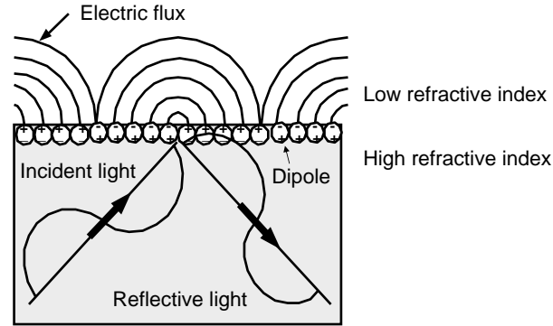
Fig. 5.2. Sketch of the near field produced at the low-refraction medium surface as the electric flux generated by dipoles due to the attenuated total reflection of light
