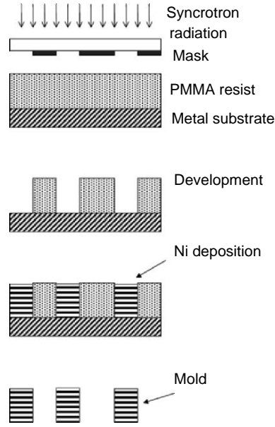
Fig. 1.6. Lithographie galvanofarming abforming (LIGA) involves X-ray lithography and electrodeposition processes
