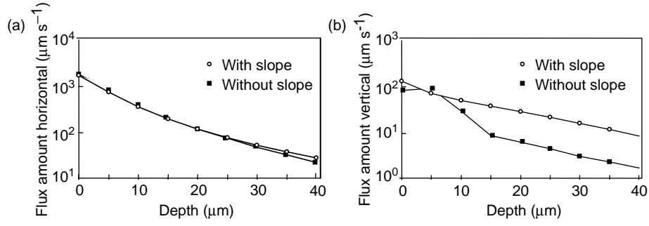
Fig. 4.26. Effect of the slope (angle of 45°) of the shuttlecock rotor on the flux amount. Horizontal (a), and vertical (b)
