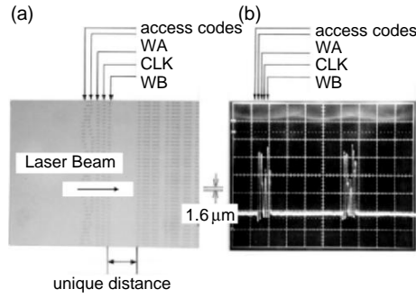
Fig. 2.37. Discrete block format (DBF) marks with a 1.6\text{-}\mu\text{m} track-pitch (a), and reproduced signals at 900 rpm. LD bias current is 40 mA (b)
