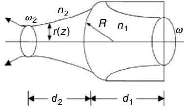
Fig. 3.17. Geometry for calculating trapping efficiency for microsphere along propagation axis by laser beam emitted from tapered lensed optical fiber
