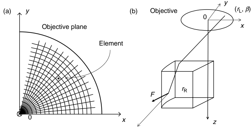
Fig. 4.5. Ray optics to simulate the optical torque of the shuttlecock rotor, where ray incidence (r_L, \beta) on the lens aperture is considered and the torque is estimated at the point r_R on side surface I
